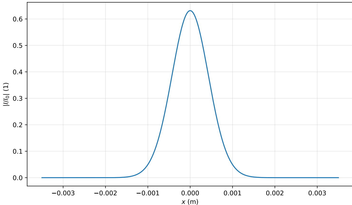
Intensity profile I(x, y = 0, z = 1.672m)/I_0 , P_{in}=0.1P_{cr} , artificial time
